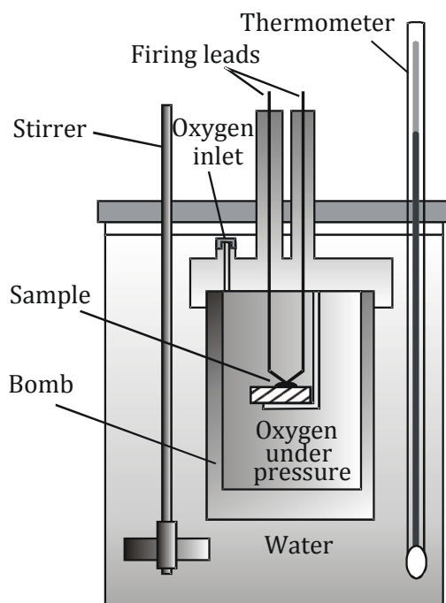
Figure : Bomb calorimeter
